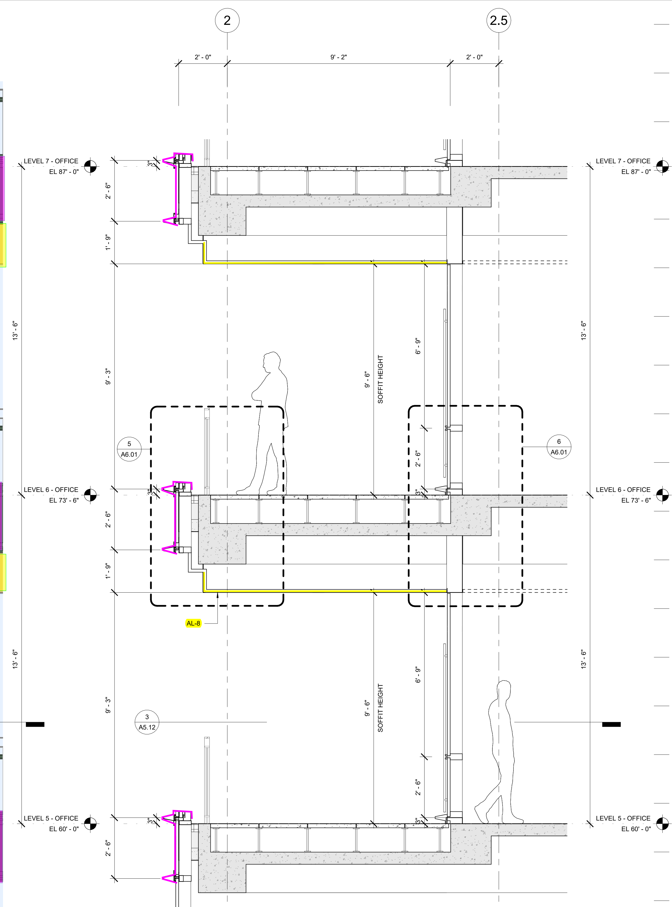
2 SECTION 1/2" = 1'-0"
