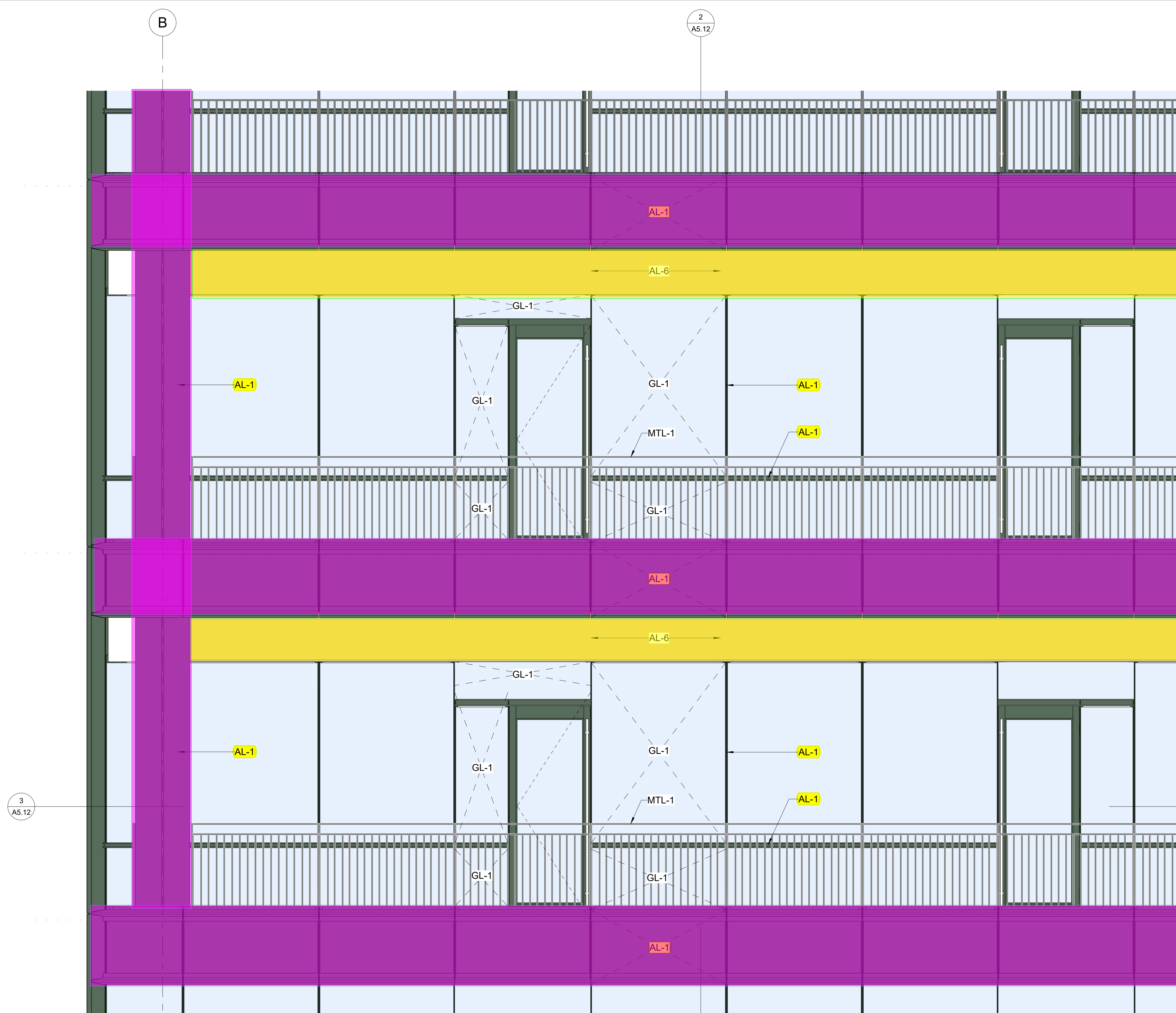
1 ELEVATION 1/2" = 1'-0"
